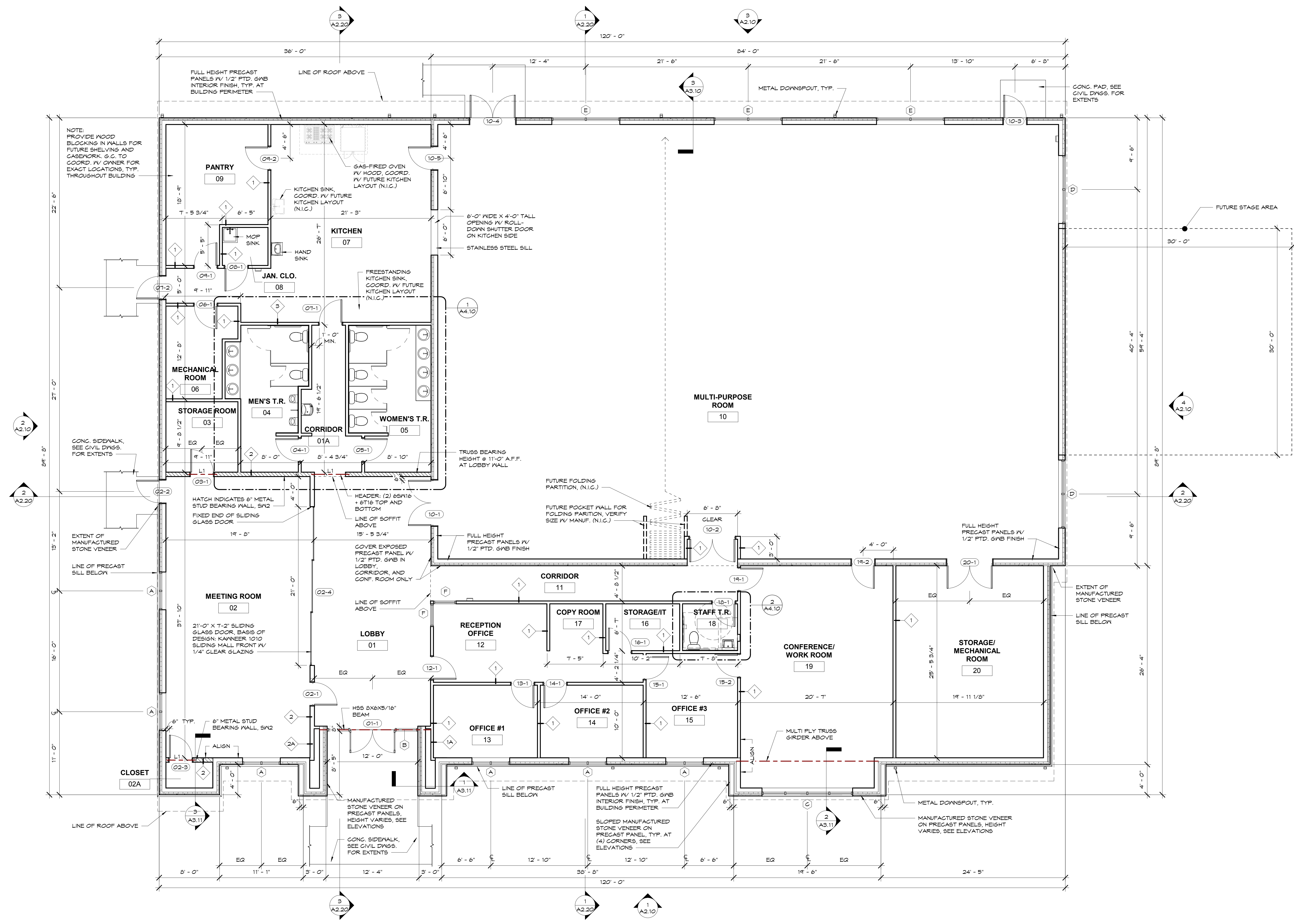
1 FIRST FLOOR PLAN 3/16" = 1'-0"
